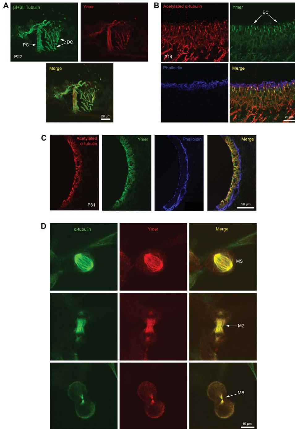
Figure 7. Colocalization studies of Ymer and different tubulins in inner ear sections and NIH-3T3 cells. A , In the mature cochlea (P22), Ymer colocalizes with (\beta 1 + \beta 2) tubulin in the cytoskeleton of PCs and Deiter's cells (DC). Similar results were obtained for \alpha -tubulin and for both acetylated and polyglutamylated tubulin (data not shown). B , In the utricle of a P14 mouse, Ymer shows spatial overlap with the cytoskeleton of microtubules in the apical cytoplasm of the epithelial cells (EC). C , In adult stria vascularis (P31), Ymer colocalizes with the microtubule-based cytoskeleton of marginal and intermediate cells. In panels B and C, no colocalization is seen with the actin cytoskeleton (phalloidin panel). D , Ymer colocalizes with microtubules of the mitotic apparatus in nontransfected NIH-3T3 cells that are undergoing cell division. In metaphase ( top panels ), Ymer distribution overlaps with microtubules of the mitotic spindle (MS). During early telophase ( middle panels ), Ymer colocalizes with the midzone (MZ), a region of bundled microtubules between the migrated chromosomes. In late telophase ( lower panels ), as the cleavage furrow ingresses compressing the midzone, Ymer colocalizes with the microtubule midbody (MB) contained in the intercellular bridge.
